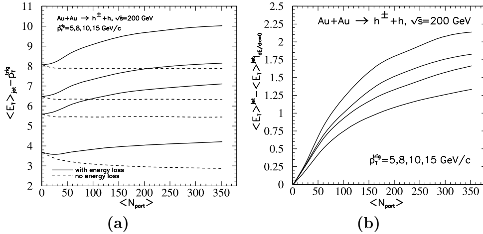
Figure 7.9: (a) Centrality dependence of \langle E_{\perp}^{jet} \rangle - p_{\perp}^{trig} from Wang analysis for p_{\perp}^{trig} = 5, 8, 10, 15 GeV/c, from top to bottom. Dashed curves represent the results with energy loss turned off in the calculation. (b) Wang prediction for the average energy loss for partons that produce a final hadron with p_{\perp}^{trig} in Au+Au collisions. p_{\perp}^{trig} increases from bottom to top. Figures taken from Ref. [70]
