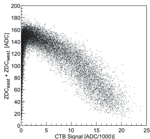
Figure 5.1: Summed ZDC vs. CTB distribution for Au+Au collisions. The lower left corner corresponds to peripheral collisions where a small amount of energy is deposited both at beam-rapidity and mid-rapidity. The lower right corner corresponds to central collisions where a small amount of energy is deposited at beam-rapidity, but a large amount of energy is deposited at mid-rapidity.
